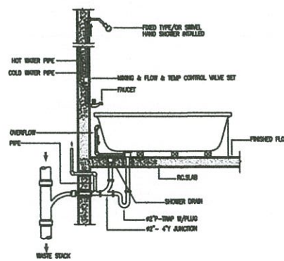
BATHTUB
