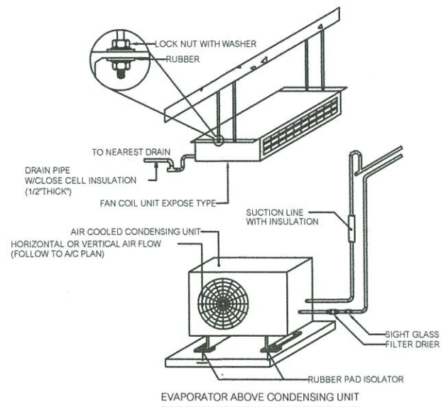
CONDENSING UNIT INSTALLATION DETAIL (FCU ABOVE CDU)
