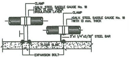
PIPE SUPPORT FOR SPLIT TYPE A/C
