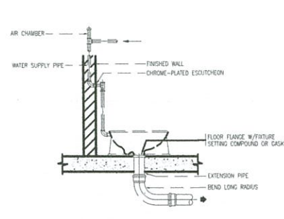
WATER CLOSET (EASTERN TYPE)
