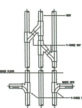
JOINTING OF SOIL-VENT-WASTE PIPE
