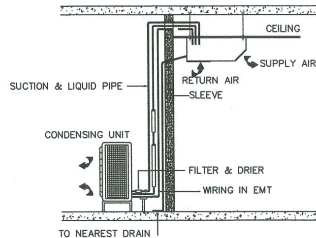
INSTALLATION OF AIR CONDITIONER (CEILING MOUNTED TYPE)
