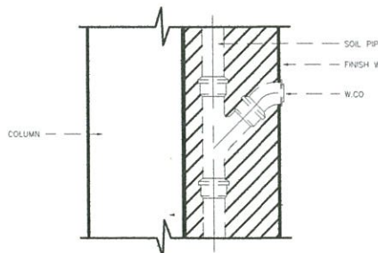
WALL CLEANOUT
