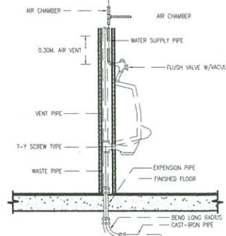
URINAL
