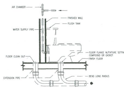
WATER CLOSET (FLUSH TANK)
