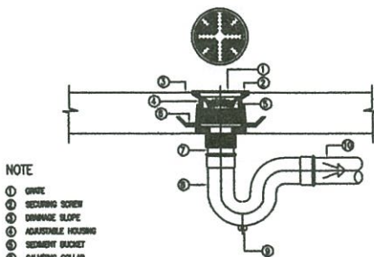
LAVATORY
