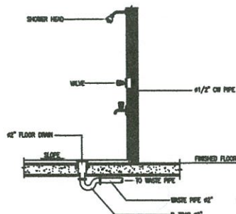
SHOWER HEAD
