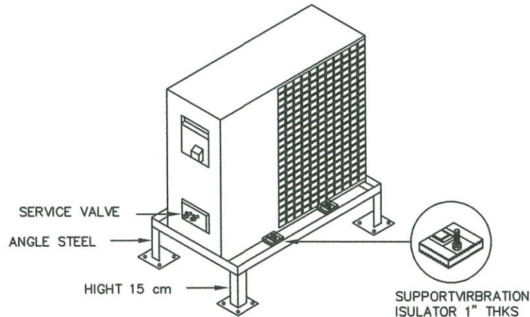
CONDENSING UNIT
