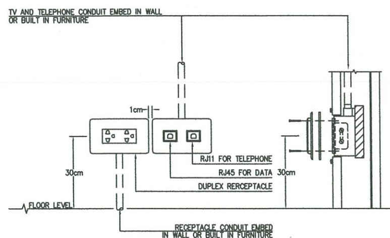
04 RECEPTACLE,TV,TELEPHONE INSTALLATION NTS
