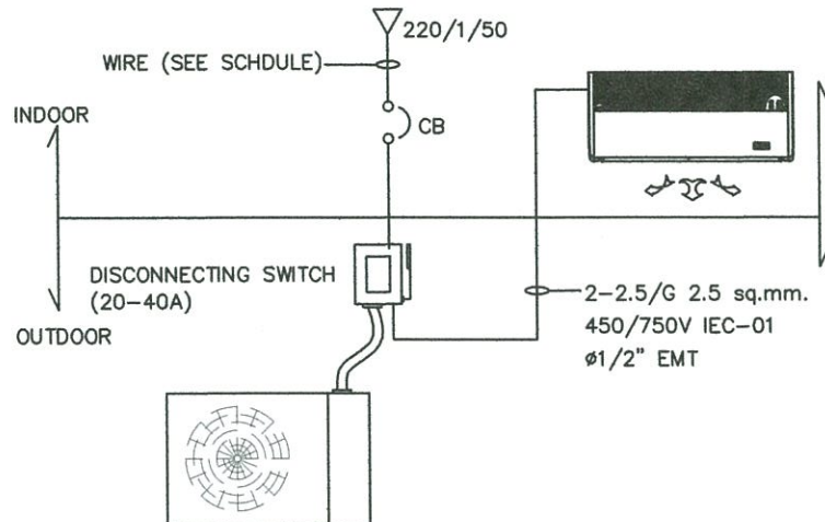
WIRING POWER SUPPLY DAIGRAM
