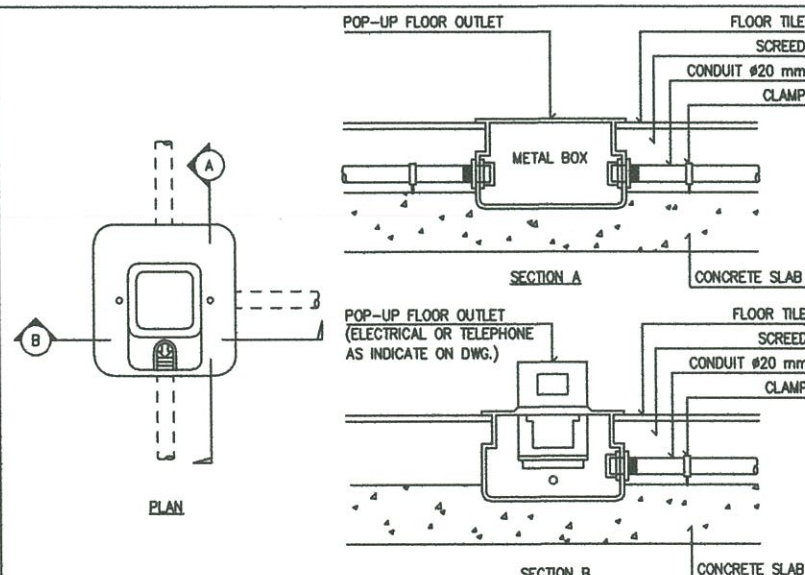
06 FLOOR OUTLET (POP-UP) NTS
