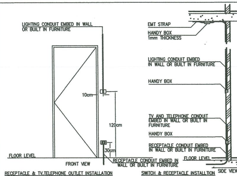
05 RECEPTACLE,TV,TELEPHONE INSTALLATION NTS
