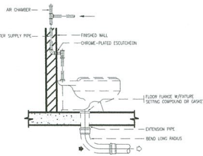
WATER CLOSET (FLUSH VALVE)
