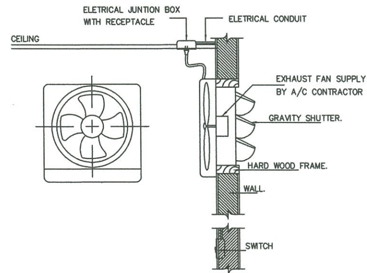
EXHAUST FAN (WALL MOUNT TYPE) EF.
