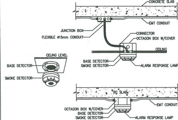
07 SMOKE DETECTOR INSTALLATION NTS
