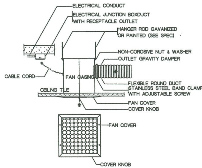
EXHAUST FAN (CEILING MOUNT TYPE) EF.
