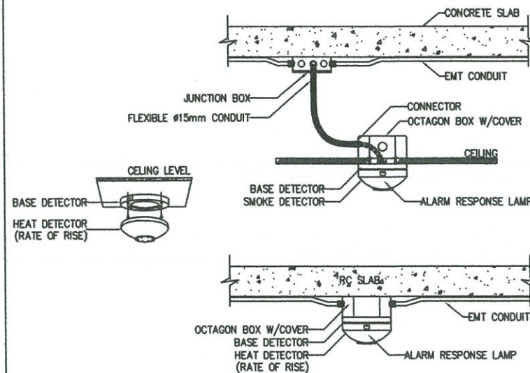
08 HEAT DETECTOR INSTALLATION NTS
